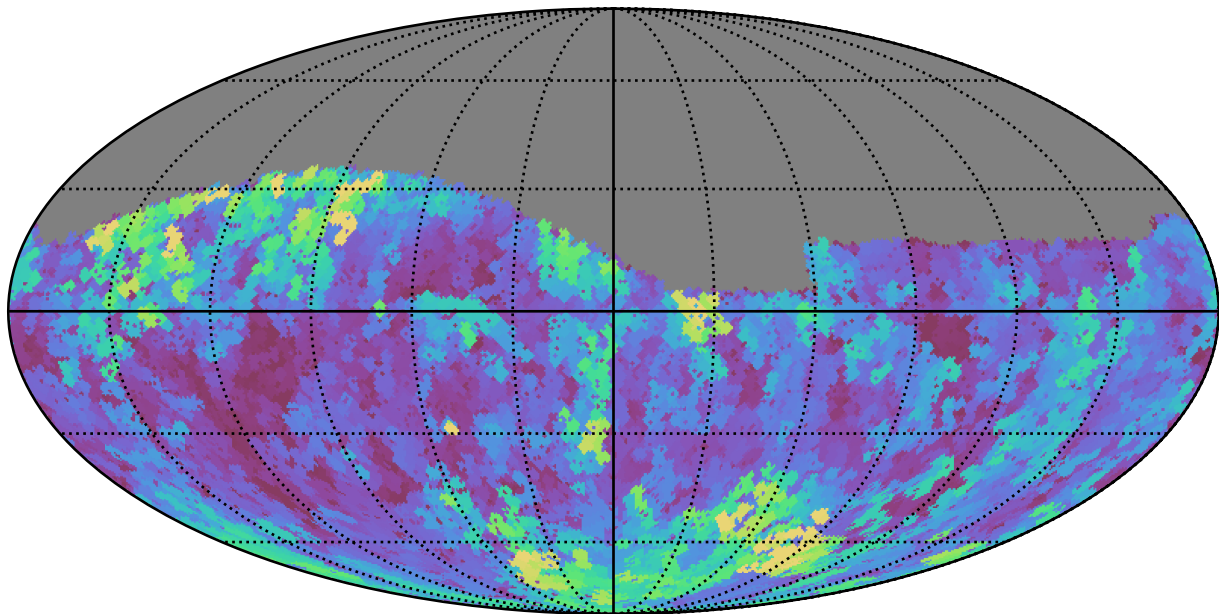
no_high_blob_v3.3_10yrs Yr 1 g band: Max seeingEff
