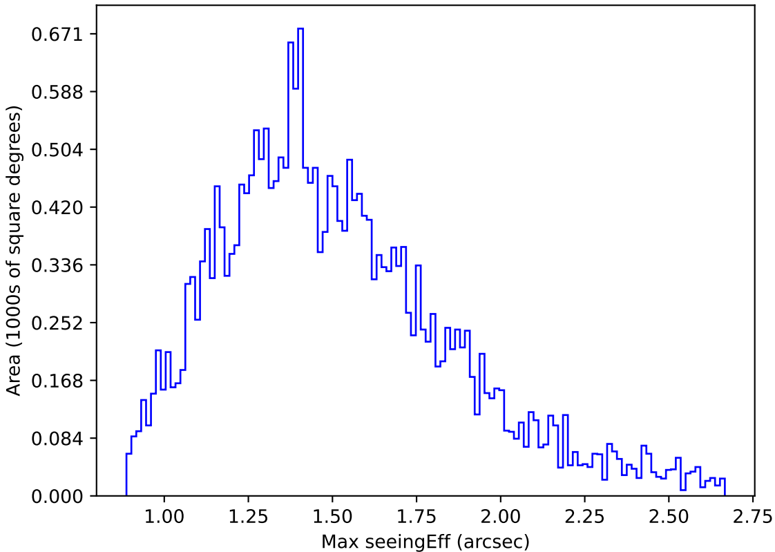
no_high_blob_v3.3_10yrs Yr 1 g band: Max seeingEff
