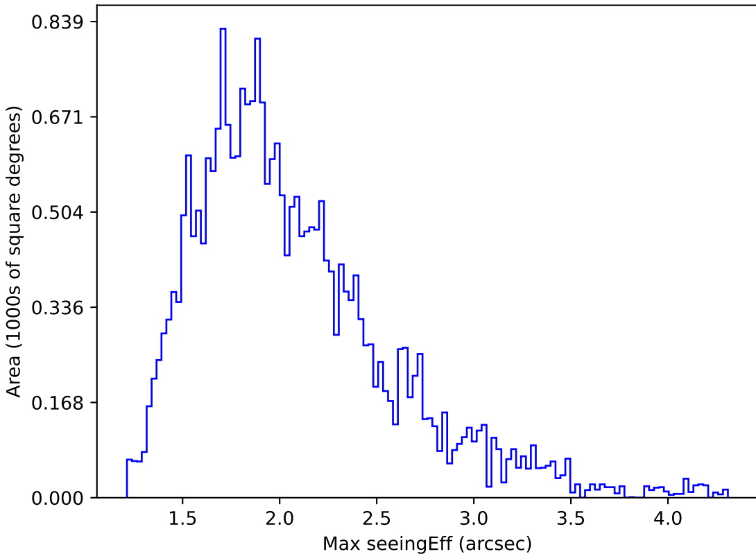
no_high_blob_v3.3_10yrs Yr 1 all bands: Max seeingEff
