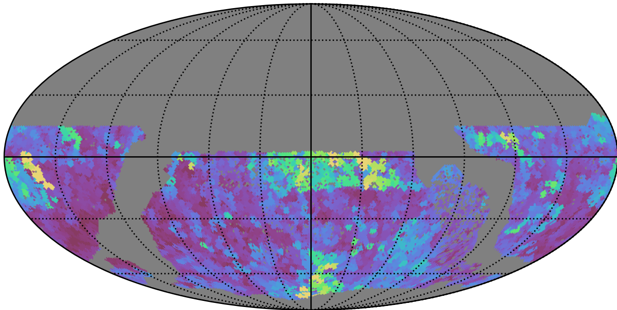
no_high_blob_v3.3_10yrs WFD z band: Max seeingEff
