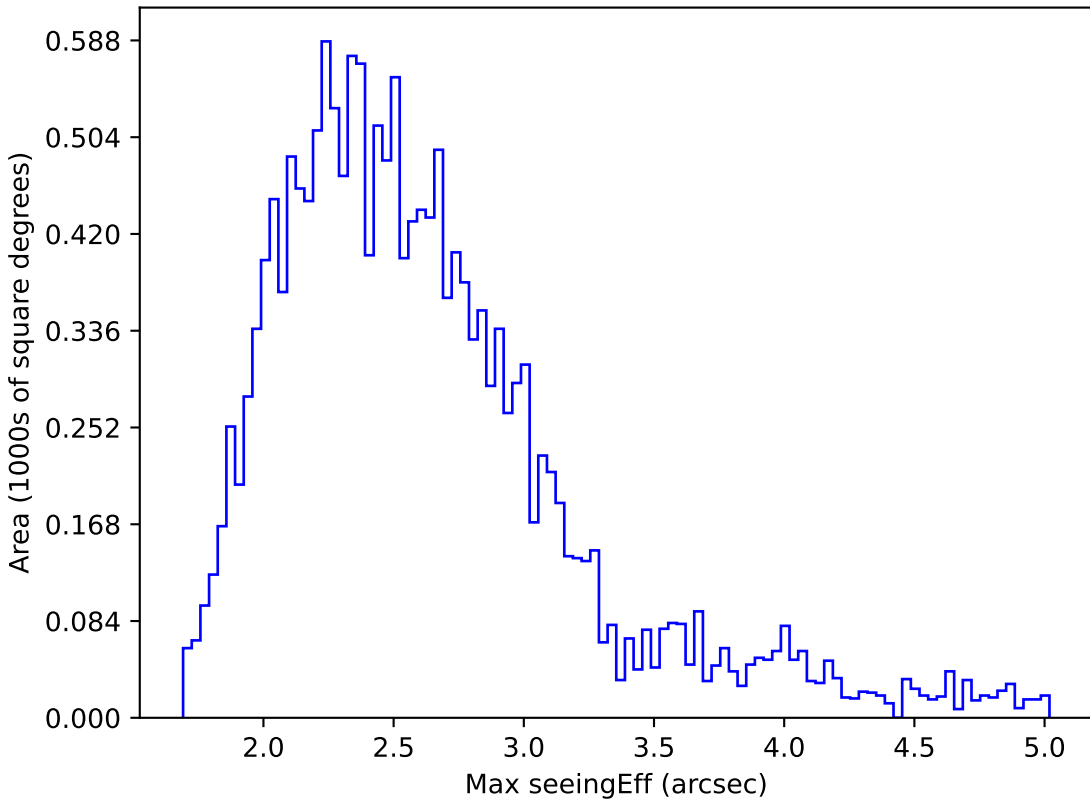
no_high_blob_v3.3_10yrs WFD z band: Max seeingEff
