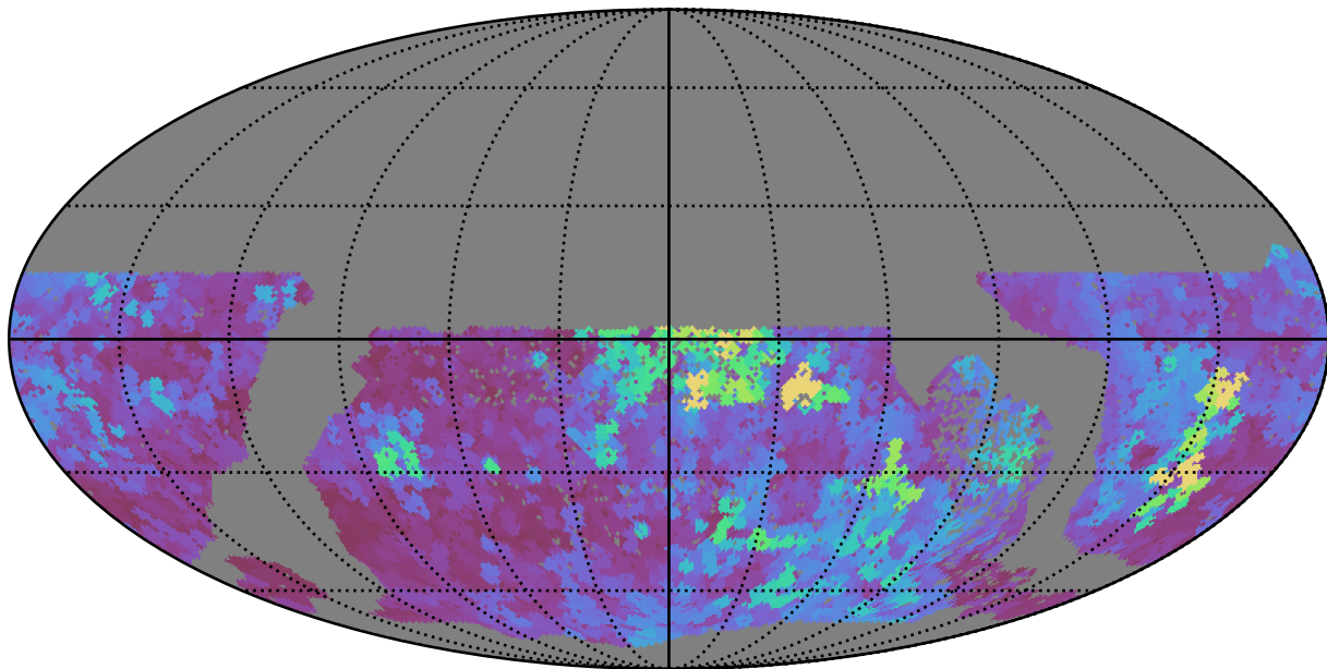
no_high_blob_v3.3_10yrs WFD y band: Max seeingEff
