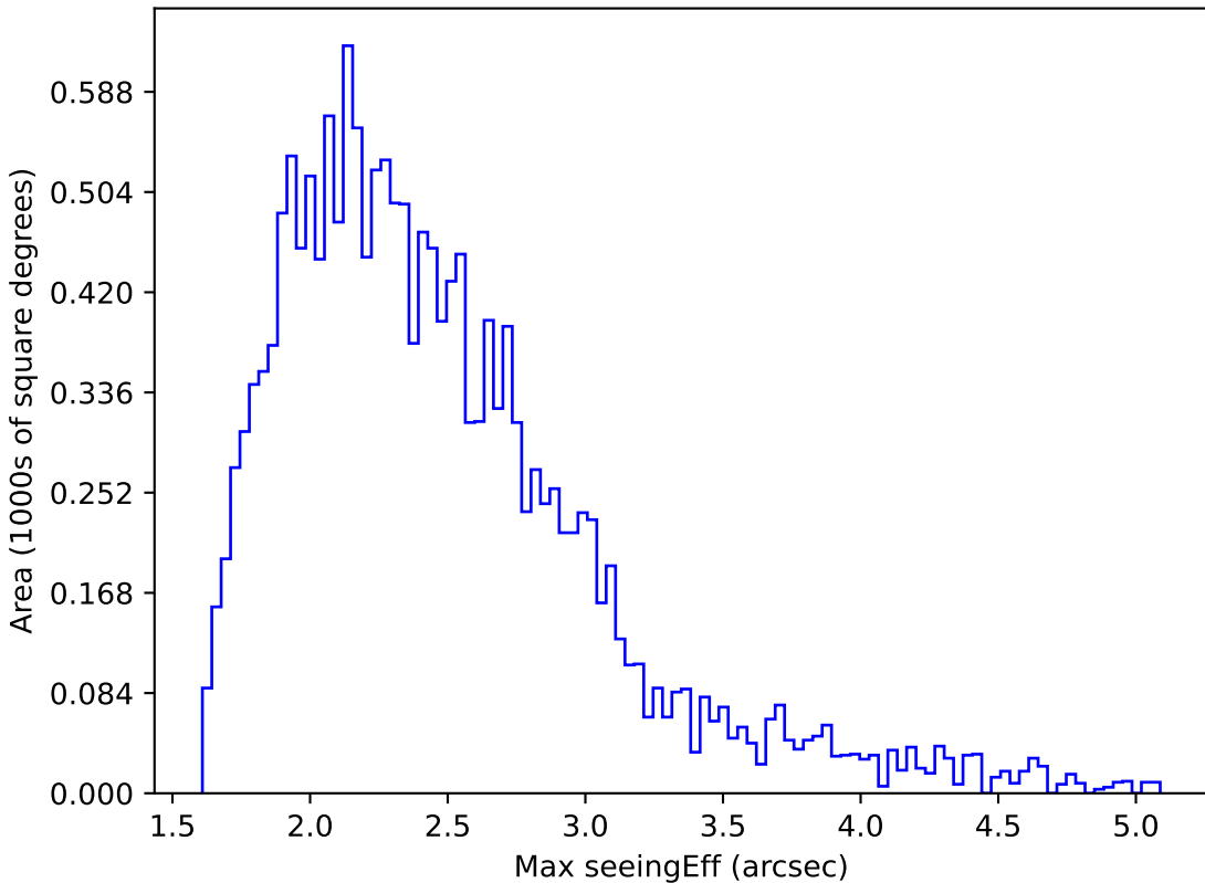
no_high_blob_v3.3_10yrs WFD y band: Max seeingEff
