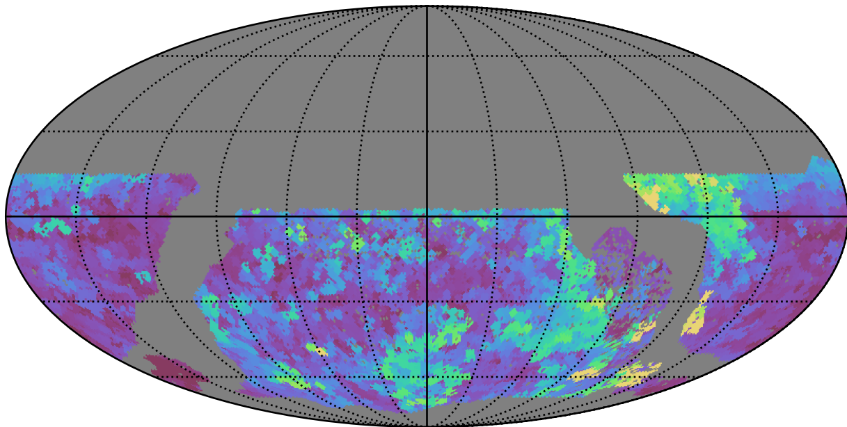
no_high_blob_v3.3_10yrs WFD u band: Max seeingEff
