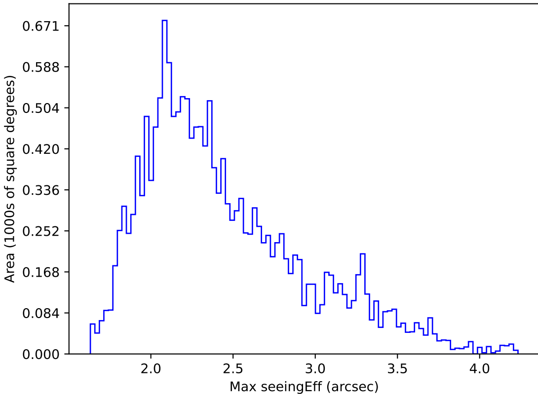
no_high_blob_v3.3_10yrs WFD u band: Max seeingEff
