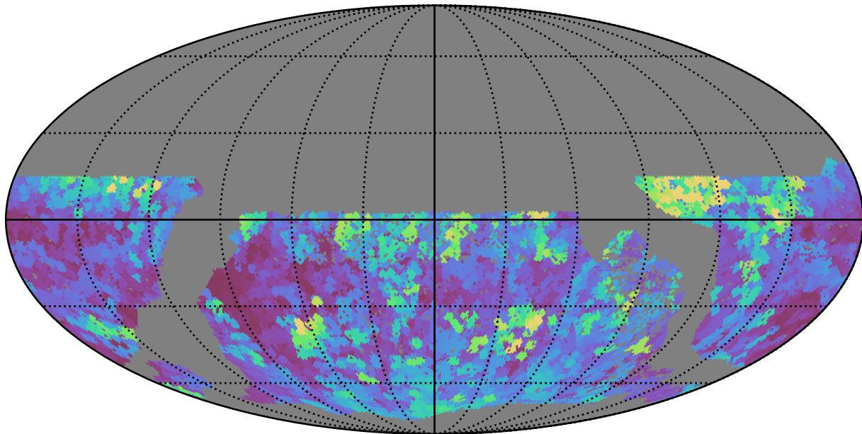
no_high_blob_v3.3_10yrs WFD r band: Max seeingEff
