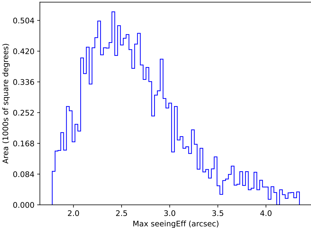
no_high_blob_v3.3_10yrs WFD r band: Max seeingEff
