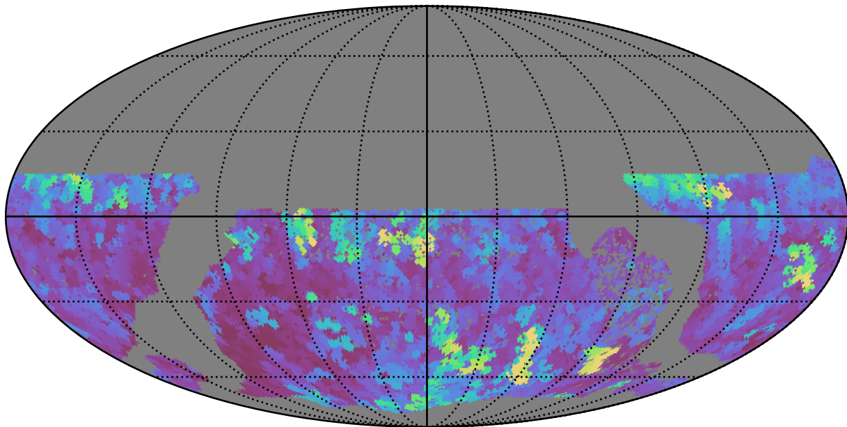
no_high_blob_v3.3_10yrs WFD i band: Max seeingEff
