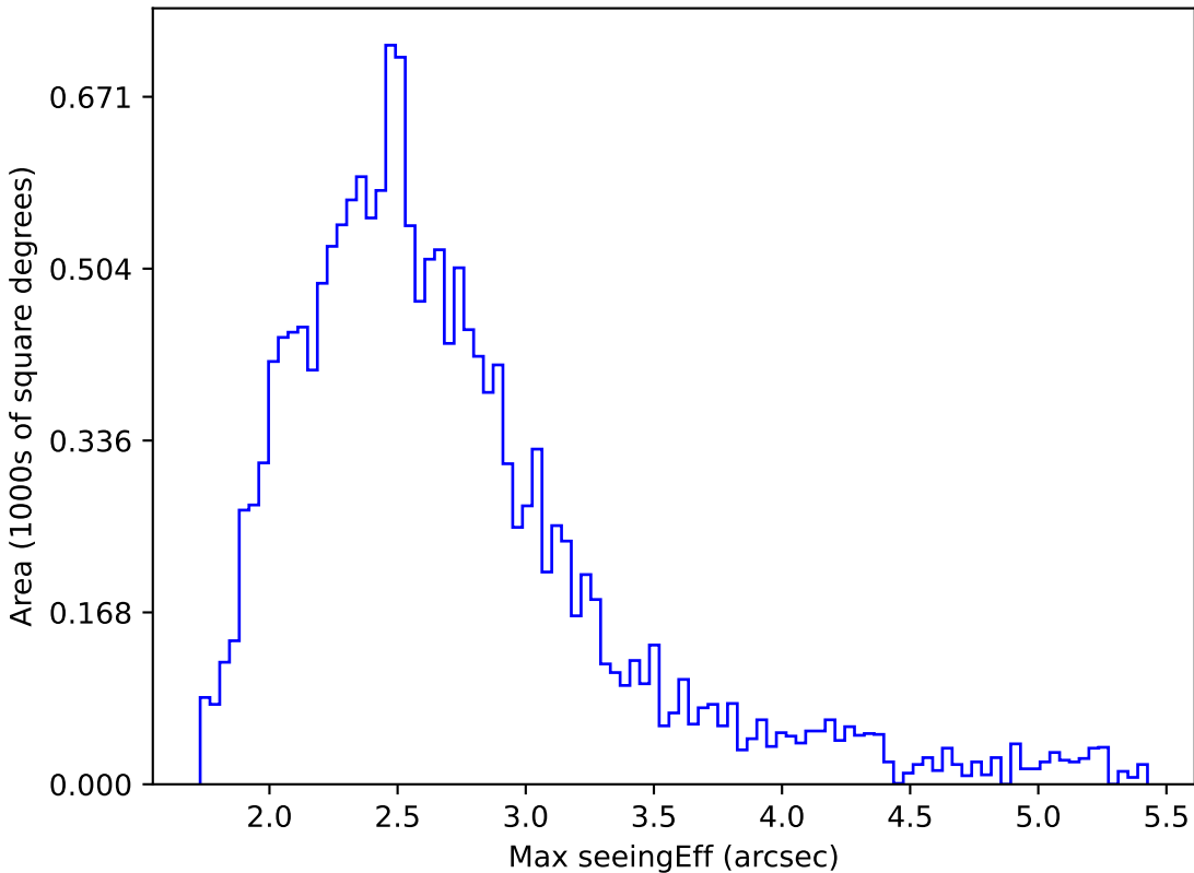
no_high_blob_v3.3_10yrs WFD i band: Max seeingEff
