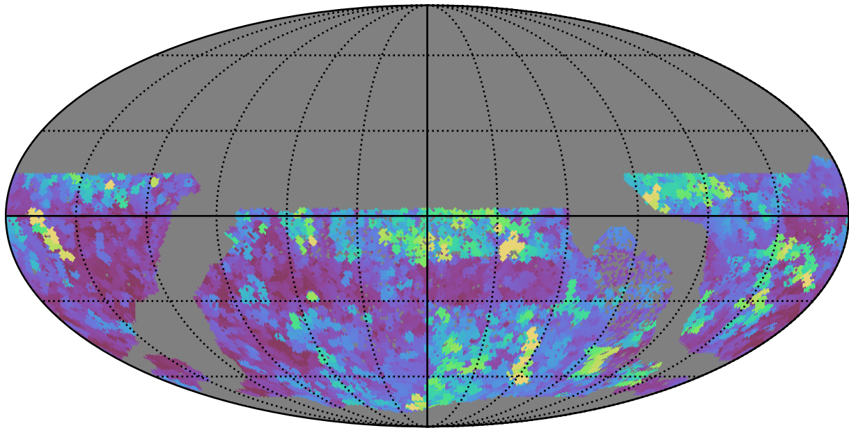
no_high_blob_v3.3_10yrs WFD all bands: Max seeingEff
