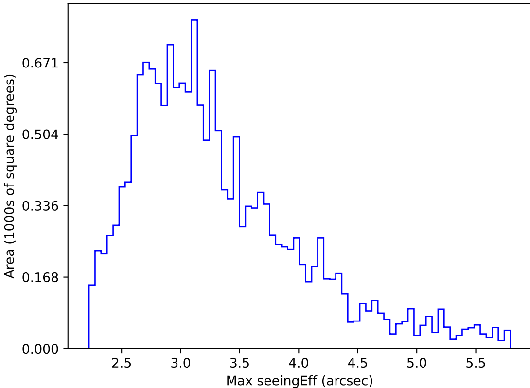
no_high_blob_v3.3_10yrs WFD all bands: Max seeingEff
