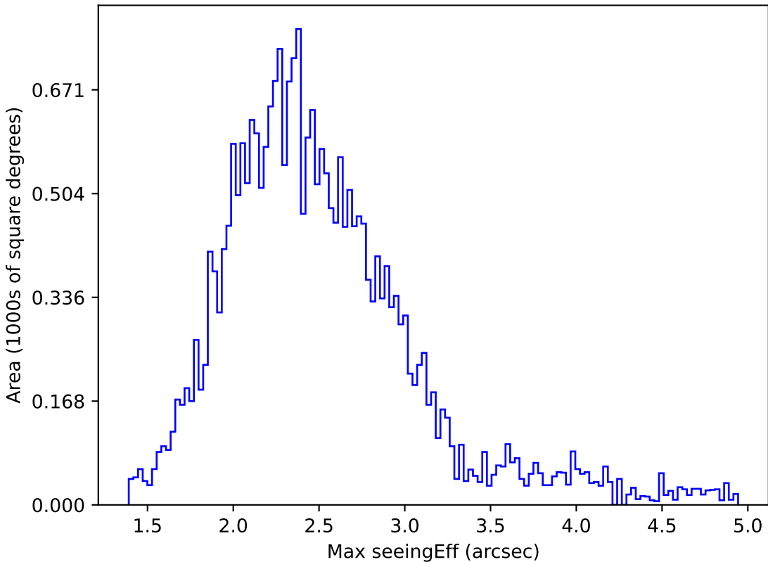
no_high_blob_v3.3_10yrs All sky z band: Max seeingEff
