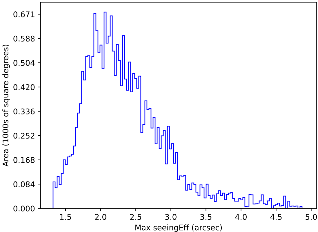
no_high_blob_v3.3_10yrs All sky y band: Max seeingEff
