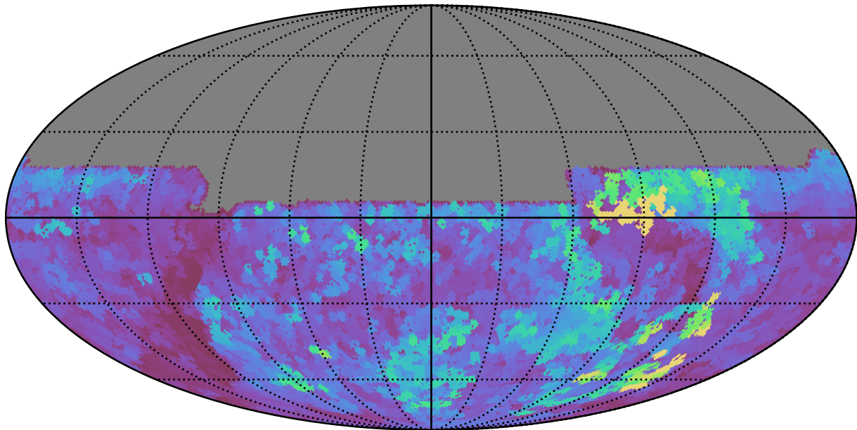
no_high_blob_v3.3_10yrs All sky u band: Max seeingEff
