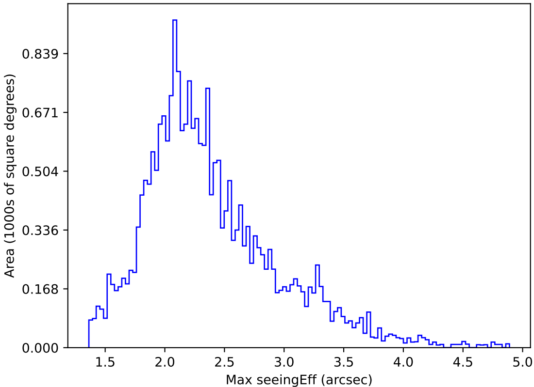
no_high_blob_v3.3_10yrs All sky u band: Max seeingEff
