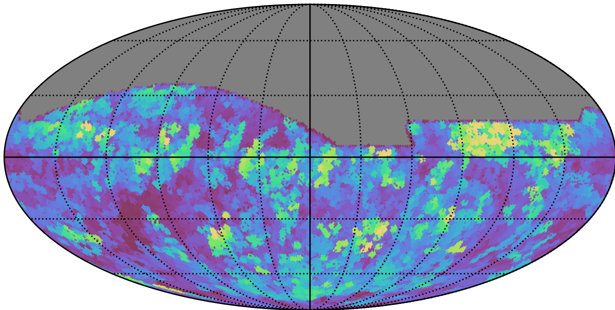
no_high_blob_v3.3_10yrs All sky r band: Max seeingEff
