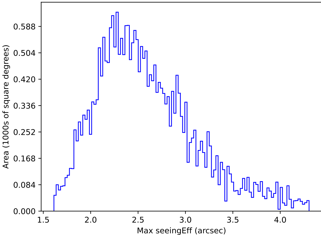
no_high_blob_v3.3_10yrs All sky r band: Max seeingEff
