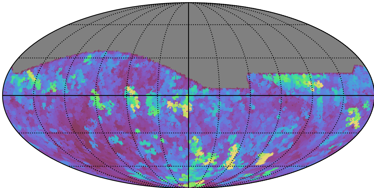
no_high_blob_v3.3_10yrs All sky i band: Max seeingEff
