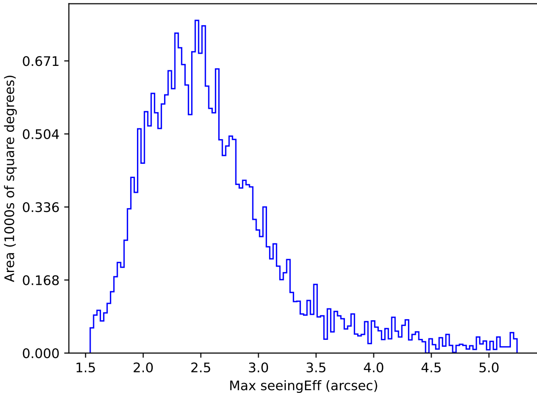
no_high_blob_v3.3_10yrs All sky i band: Max seeingEff
