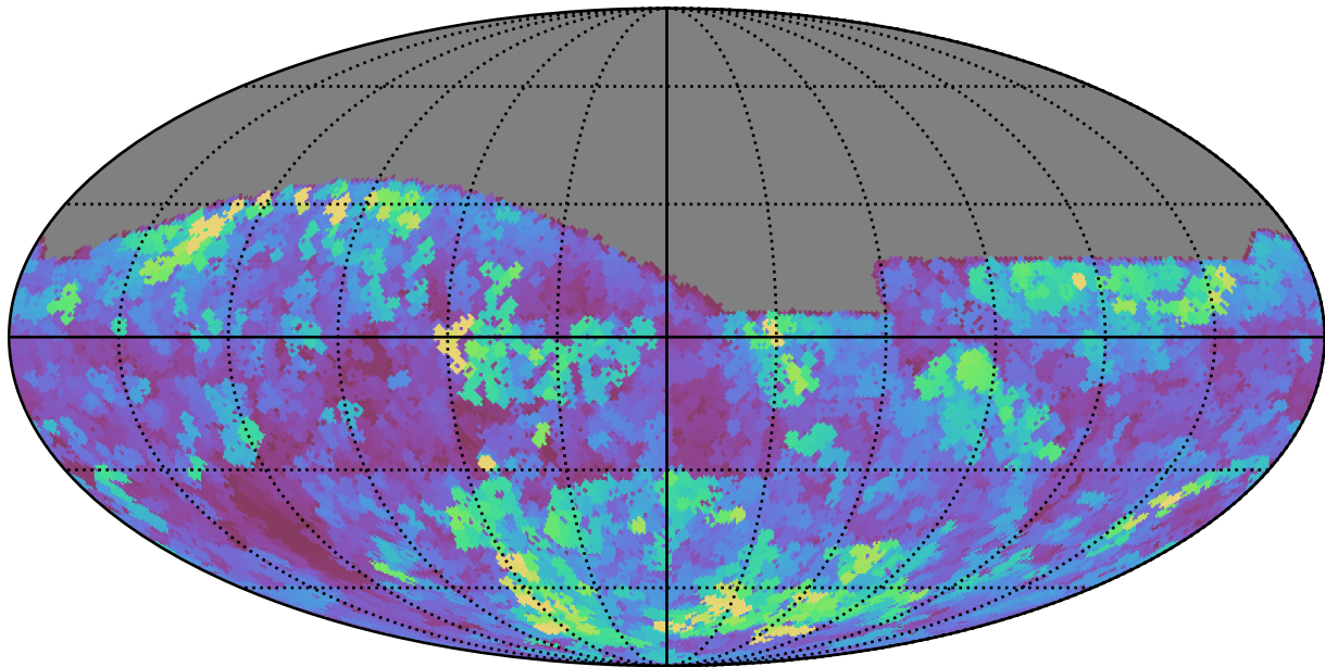
no_high_blob_v3.3_10yrs All sky g band: Max seeingEff
