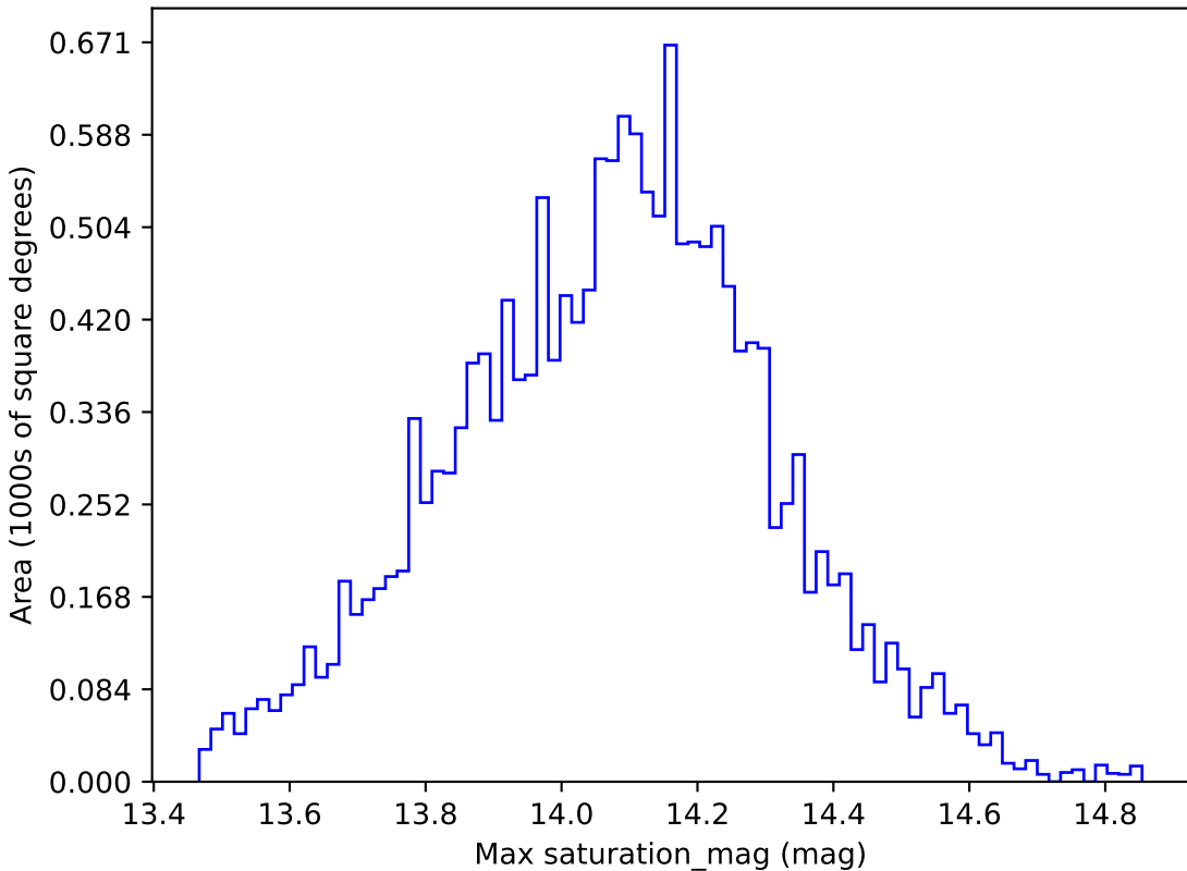
no_high_blob_v3.3_10yrs WFD u band: Max saturation_mag
