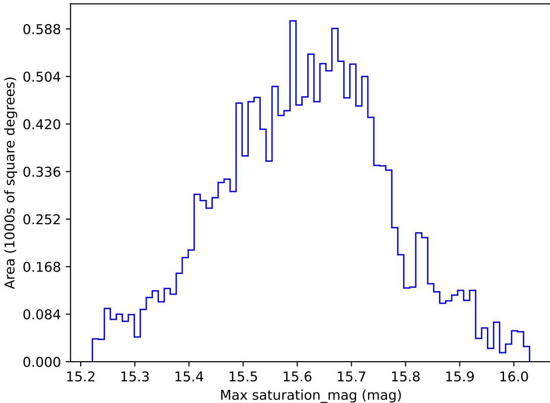
no_high_blob_v3.3_10yrs WFD i band: Max saturation_mag
