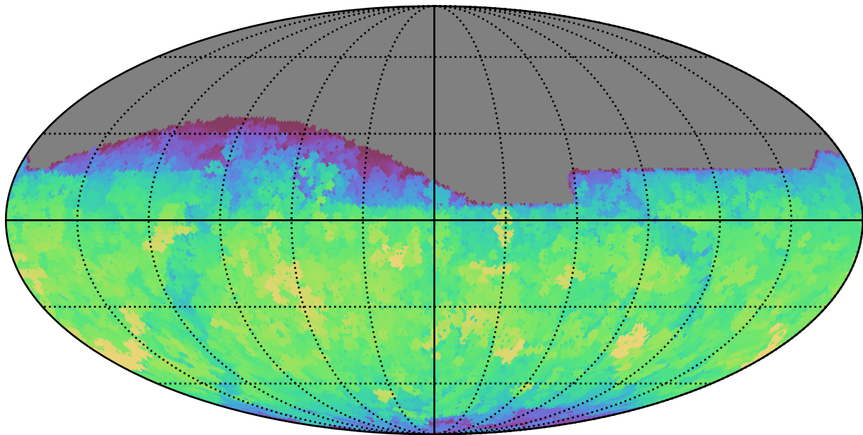
no_high_blob_v3.3_10yrs All sky z band: Max saturation_mag
