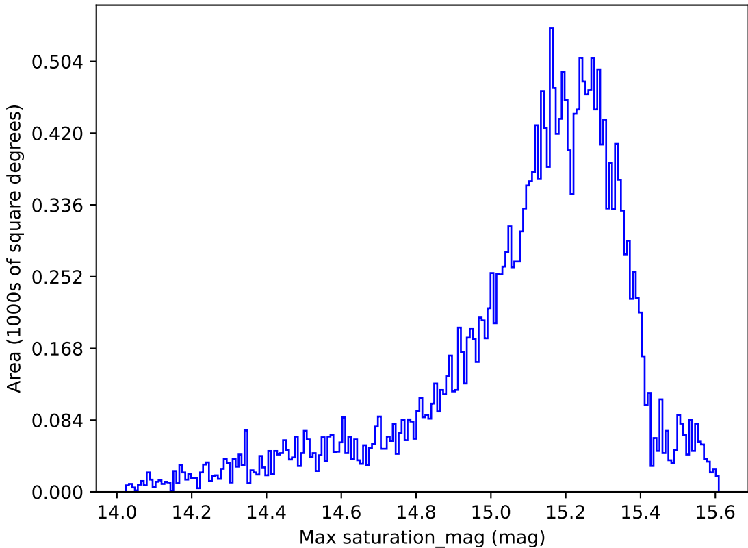
no_high_blob_v3.3_10yrs All sky z band: Max saturation_mag
