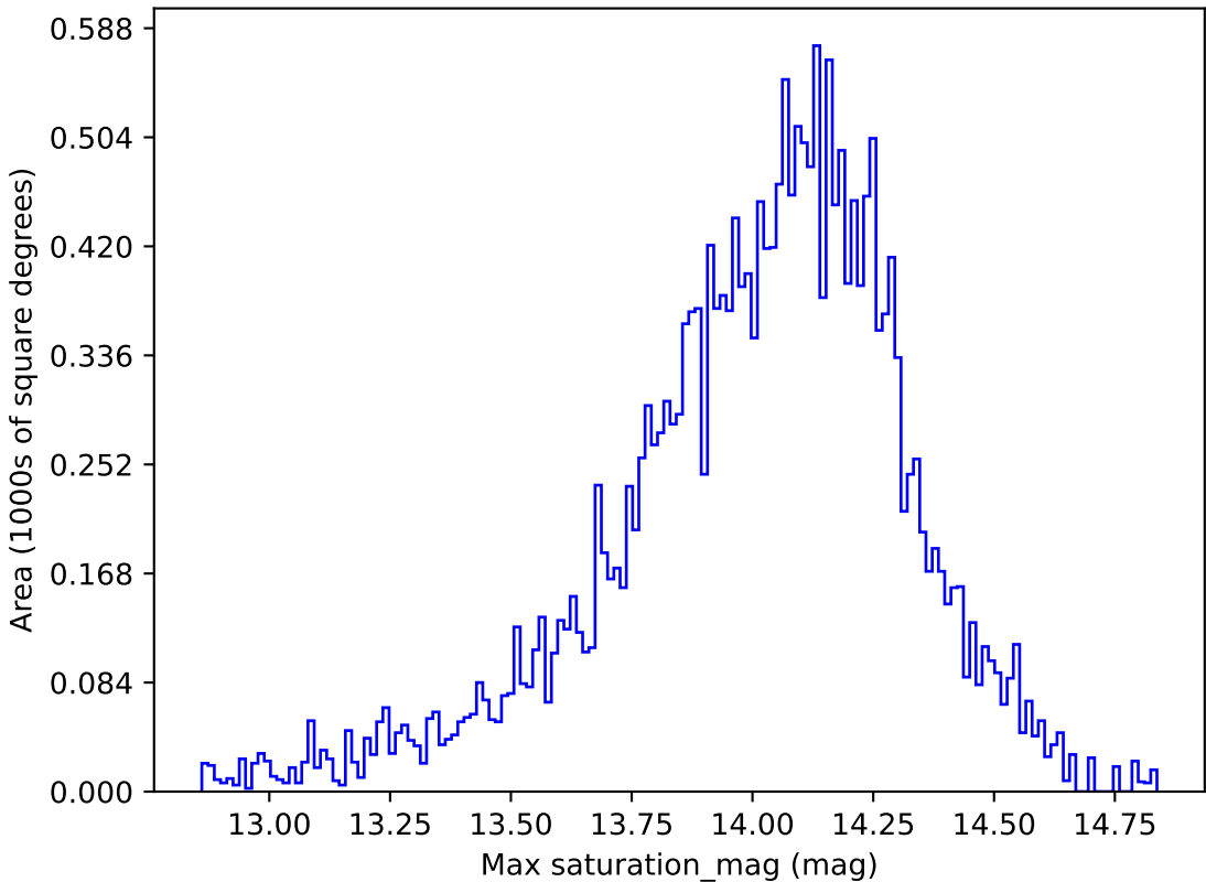
no_high_blob_v3.3_10yrs All sky u band: Max saturation_mag
