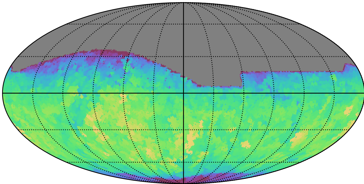
no_high_blob_v3.3_10yrs All sky i band: Max saturation_mag
