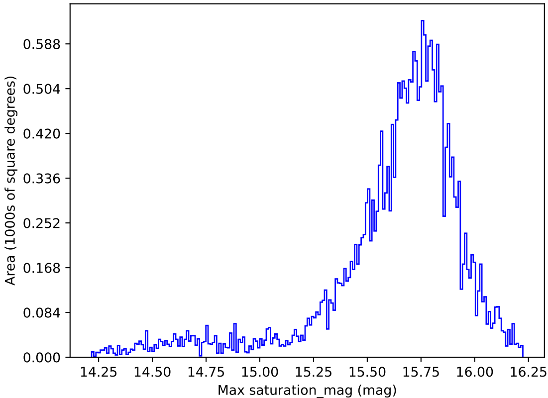
no_high_blob_v3.3_10yrs All sky g band: Max saturation_mag
