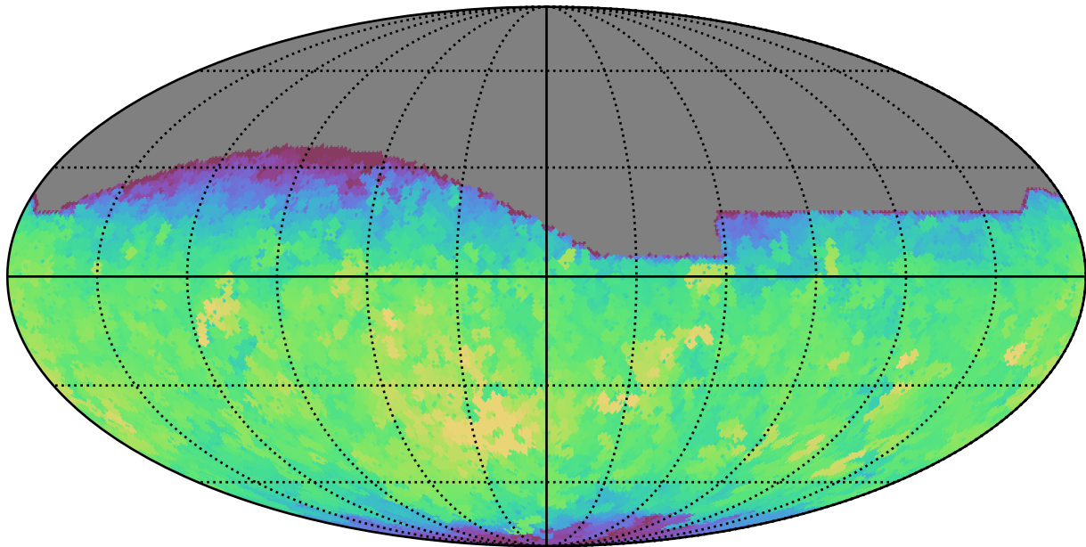
no_high_blob_v3.3_10yrs All sky all bands: Max saturation_mag
