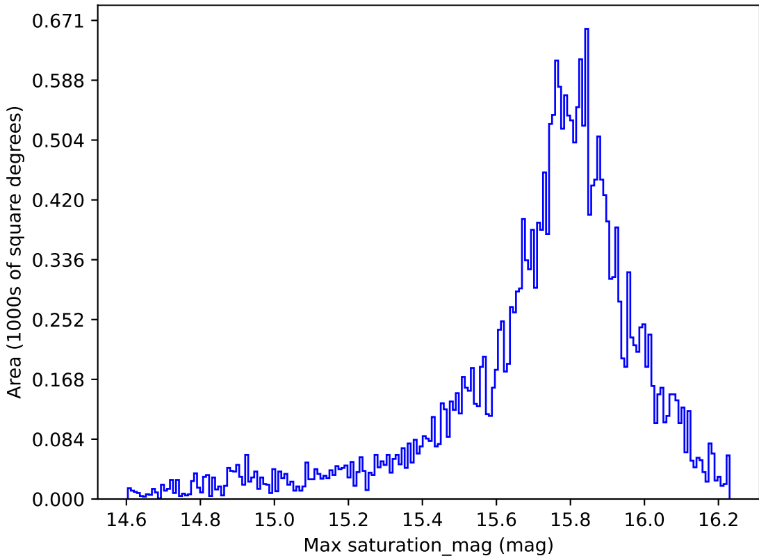
no_high_blob_v3.3_10yrs All sky all bands: Max saturation_mag
