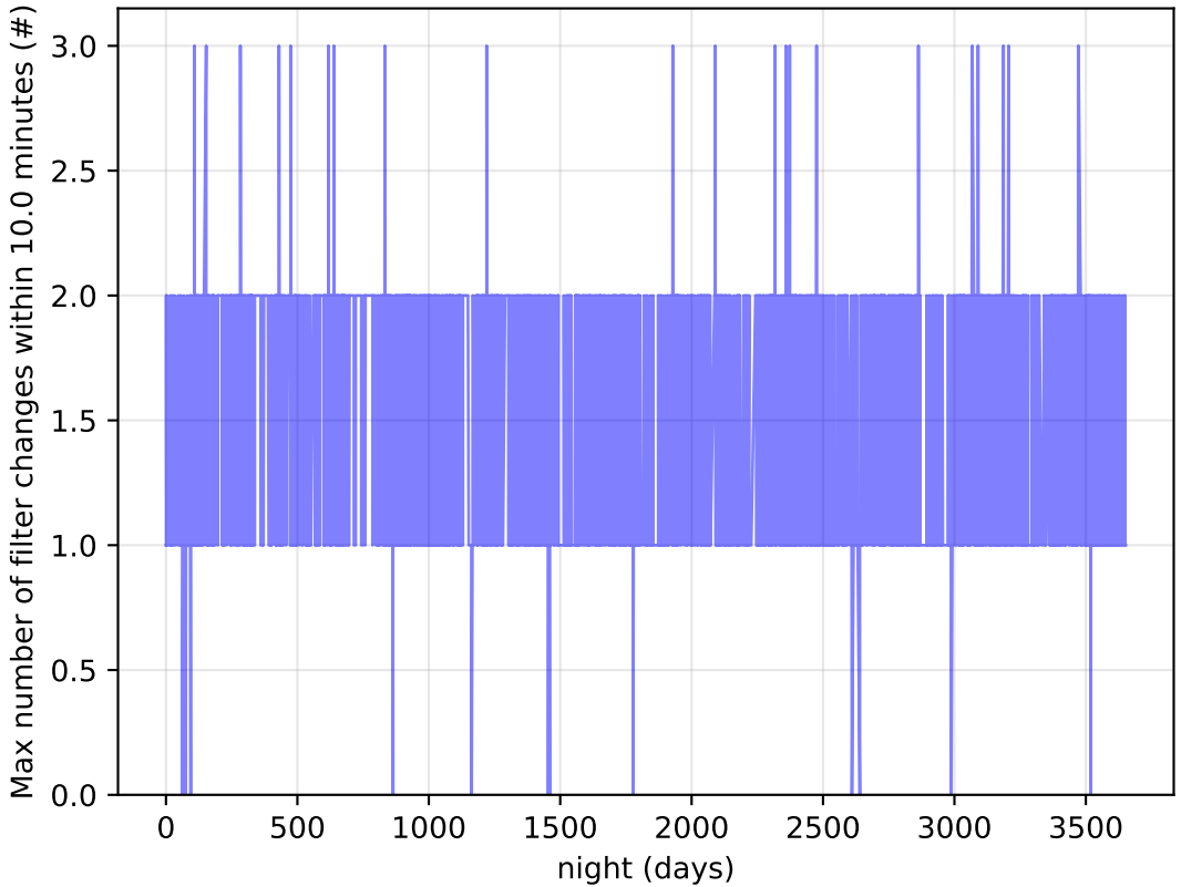
no_high_blob_v3.3_10yrs Per Night: Max number of filter changes within 10.0 minutes
