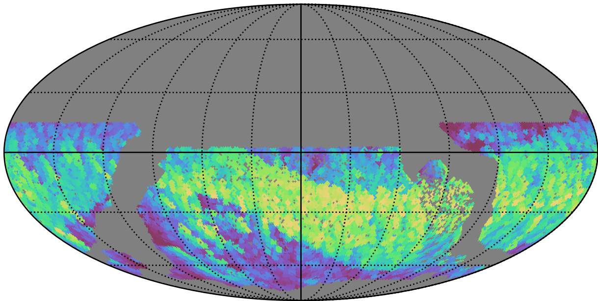
no_high_blob_v3.3_10yrs WFD z band: Max normairmass
