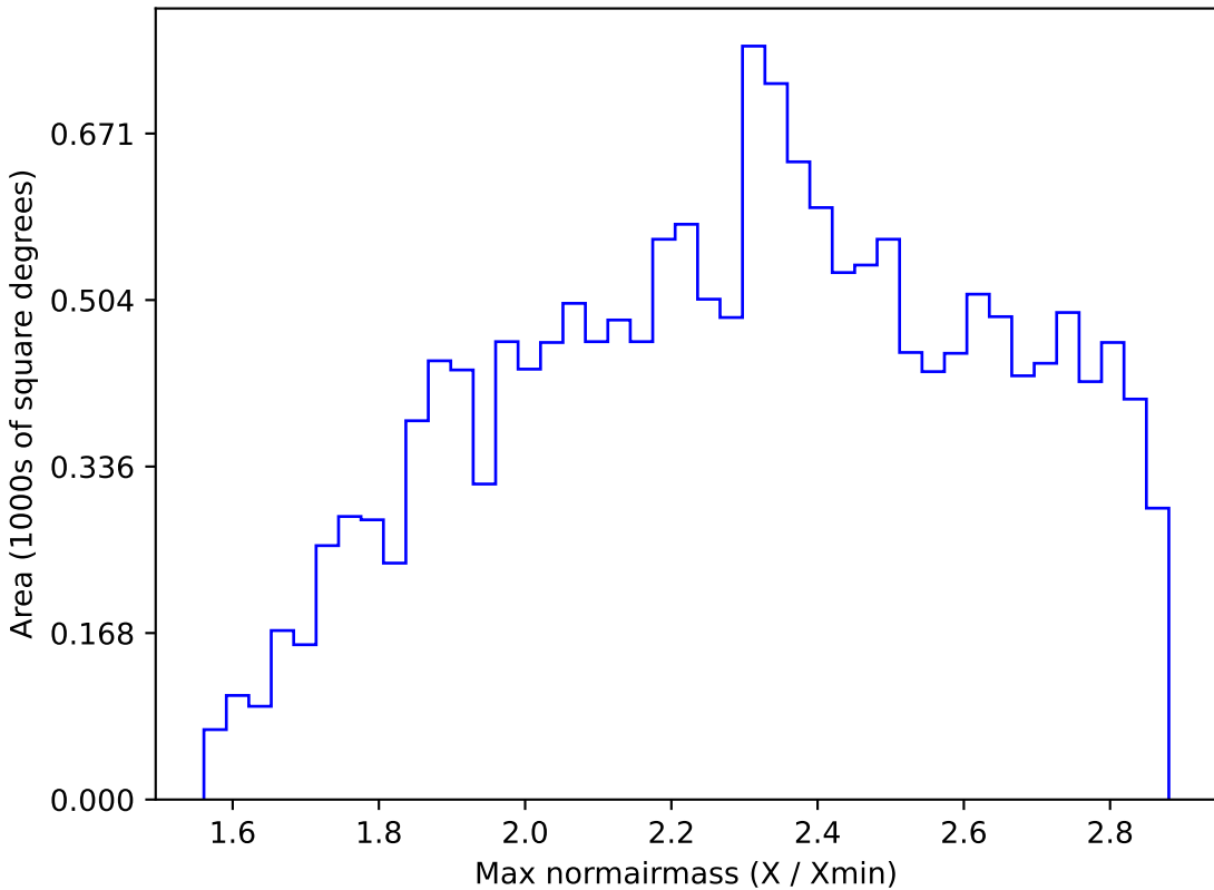
no_high_blob_v3.3_10yrs WFD z band: Max normairmass
