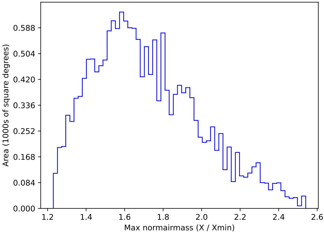
no_high_blob_v3.3_10yrs WFD u band: Max normairmass
