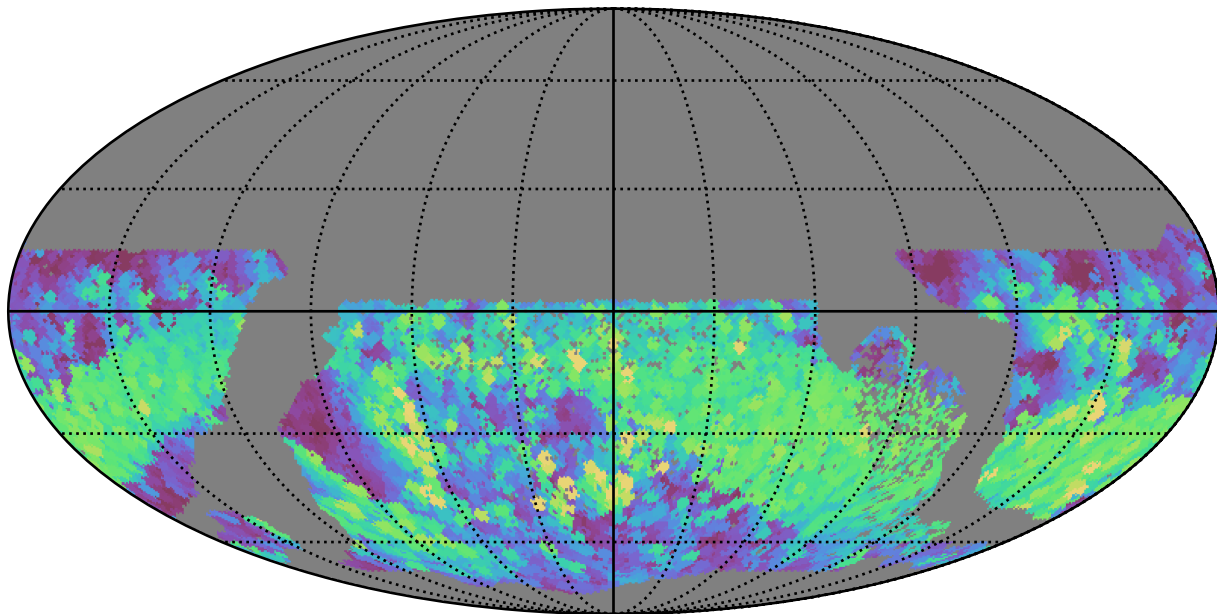
no_high_blob_v3.3_10yrs WFD r band: Max normairmass
