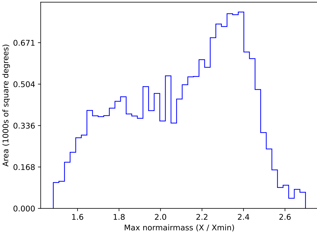
no_high_blob_v3.3_10yrs WFD r band: Max normairmass
