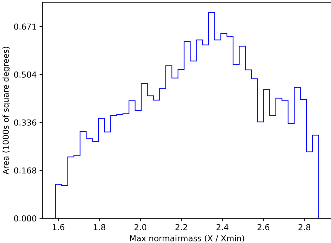
no_high_blob_v3.3_10yrs WFD i band: Max normairmass
