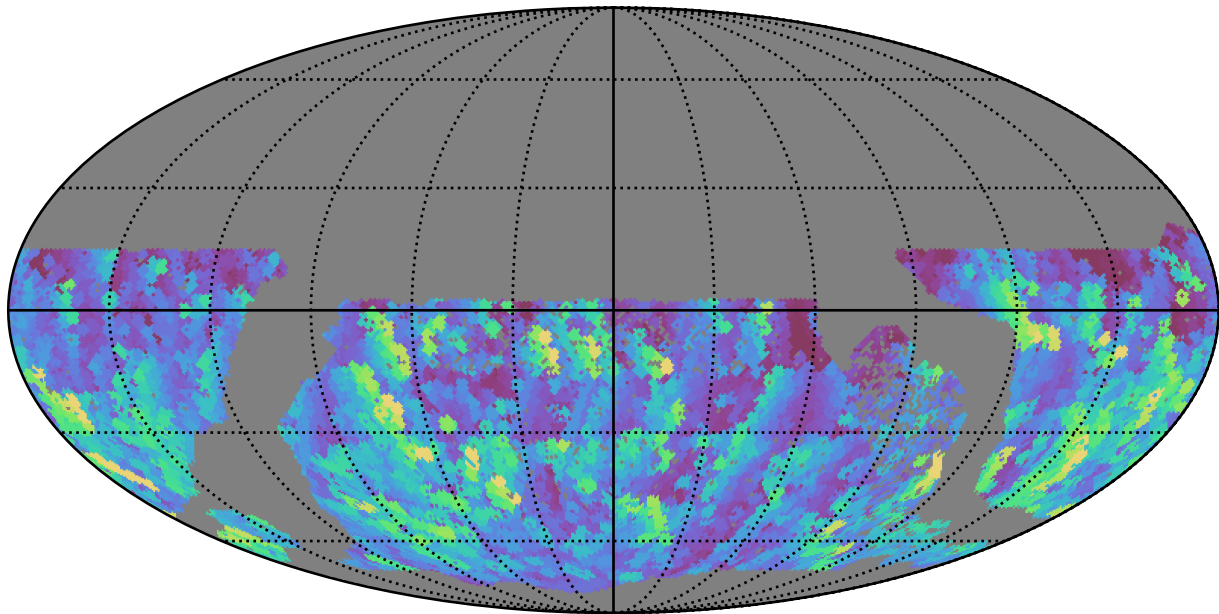
no_high_blob_v3.3_10yrs WFD g band: Max normairmass
