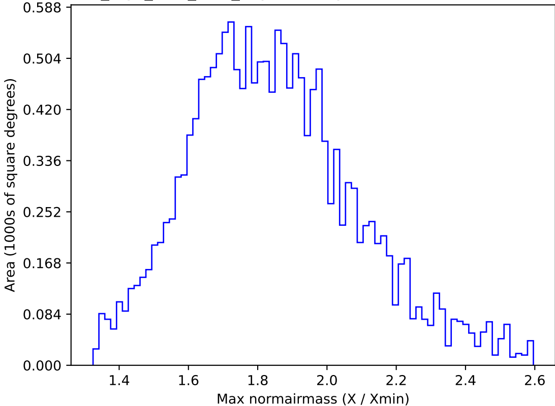
no_high_blob_v3.3_10yrs WFD g band: Max normairmass
