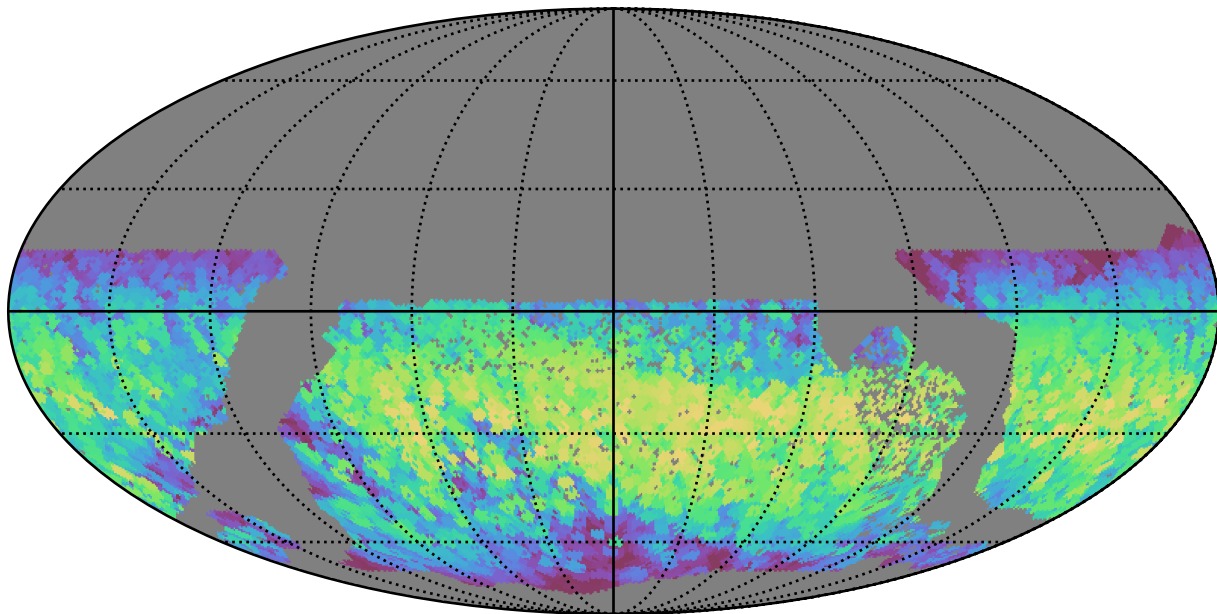
no_high_blob_v3.3_10yrs WFD all bands: Max normairmass
