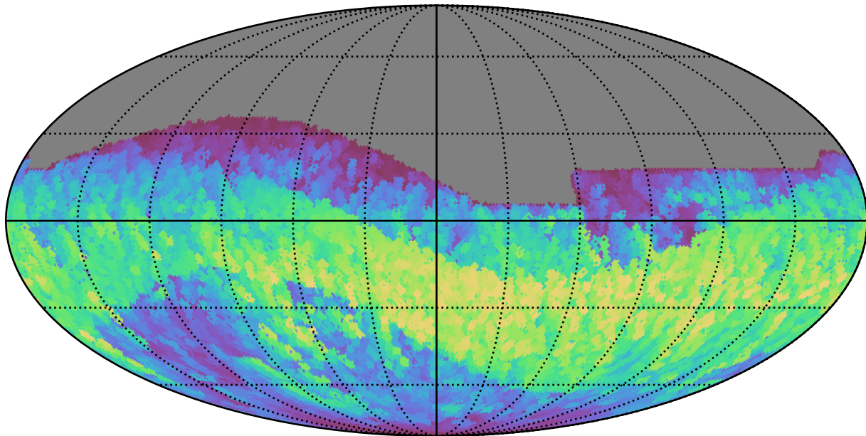
no_high_blob_v3.3_10yrs All sky z band: Max normairmass
