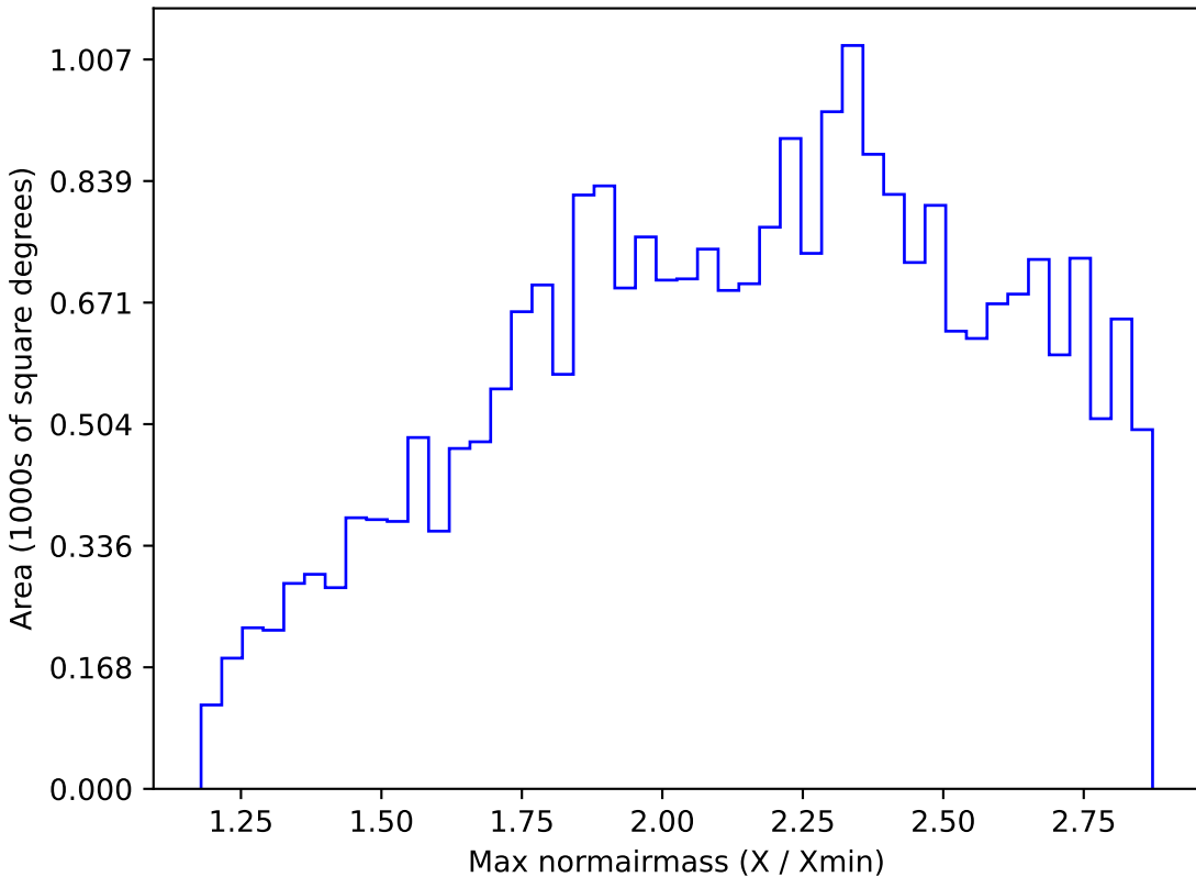
no_high_blob_v3.3_10yrs All sky z band: Max normairmass
