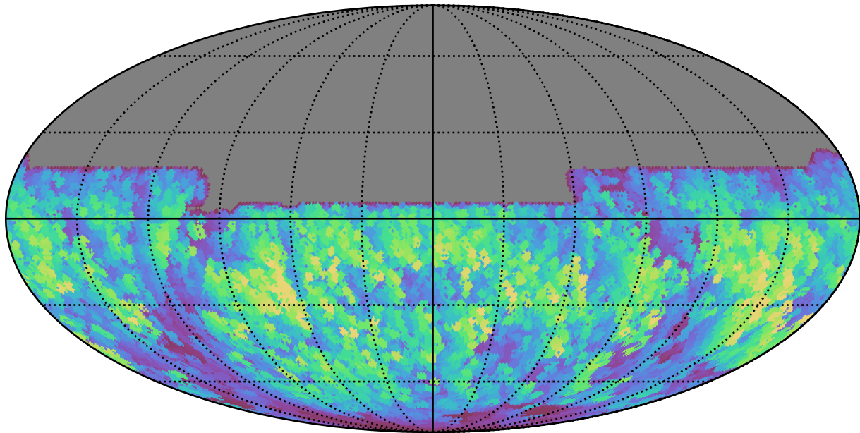
no_high_blob_v3.3_10yrs All sky y band: Max normairmass
