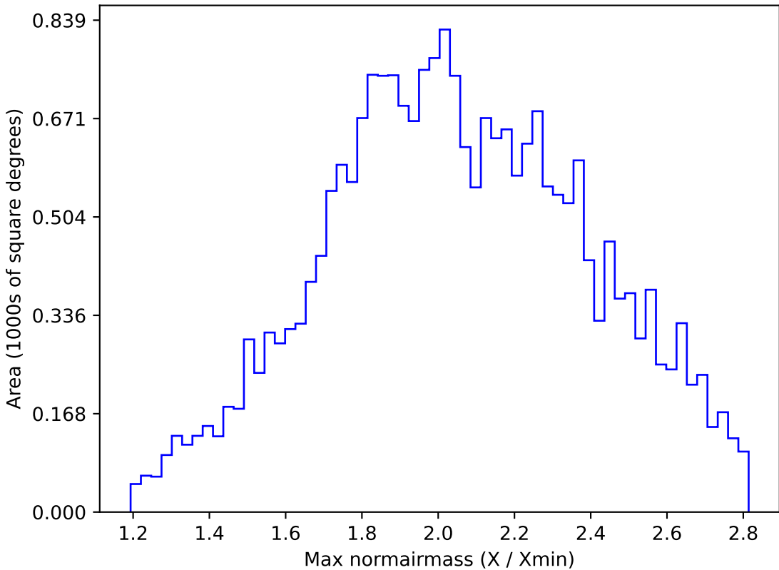
no_high_blob_v3.3_10yrs All sky y band: Max normairmass
