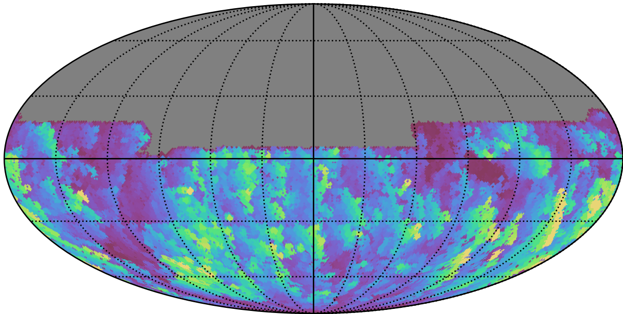
no_high_blob_v3.3_10yrs All sky u band: Max normairmass
