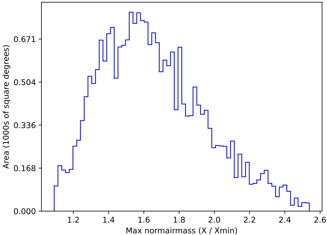
no_high_blob_v3.3_10yrs All sky u band: Max normairmass
