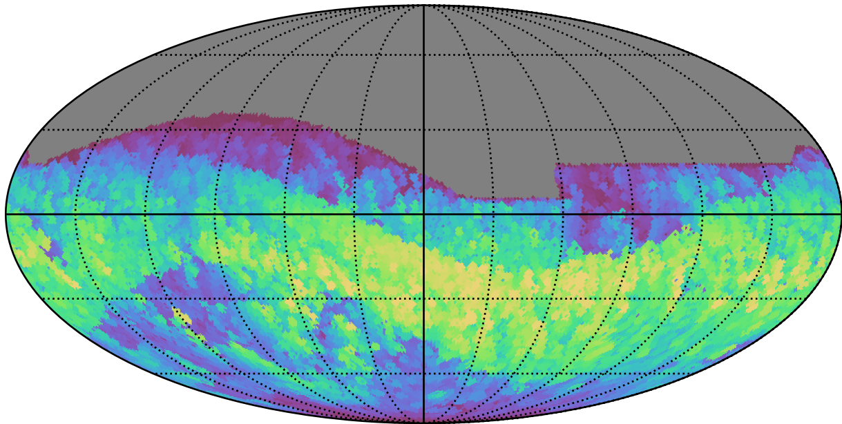
no_high_blob_v3.3_10yrs All sky i band: Max normairmass
